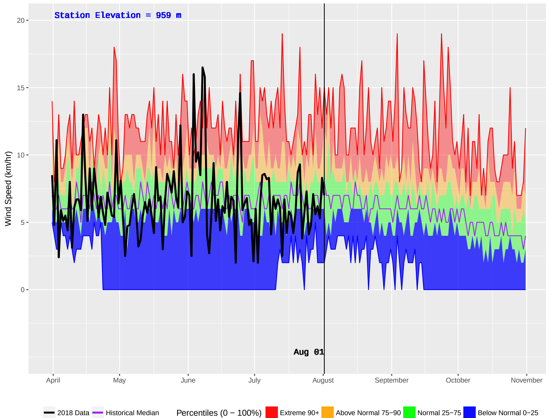
WELLS GRAY (266) : Historical (1994–2016) and Current (2018) Daily Wind Speed
